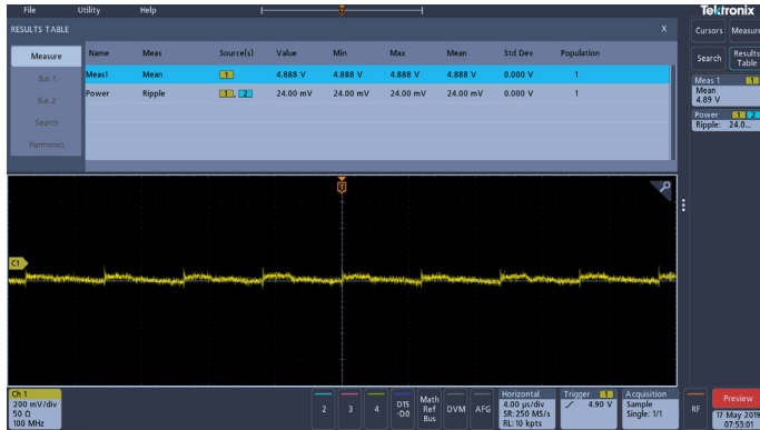
Figure 16. Ripple Measurements.
