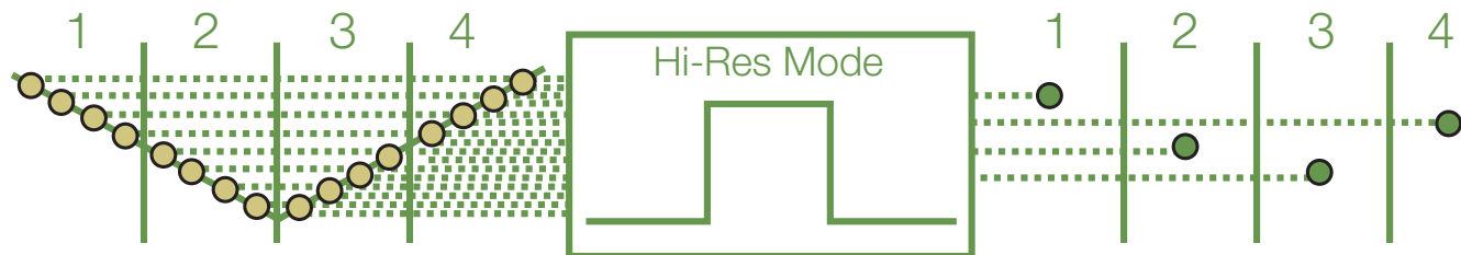
Figure 4. Hi Res Mode.
