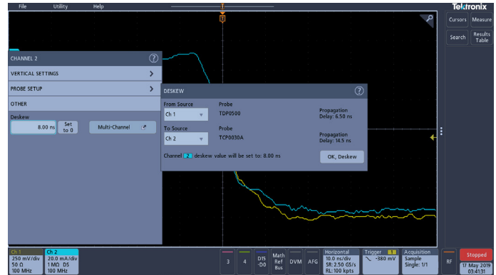
Figure 6. Nominal Correction of Timing Skew between Voltage and Current Probes.
