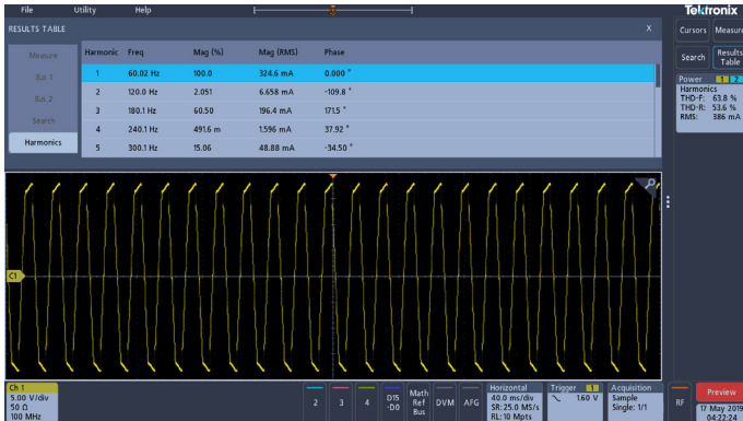
Figure 10. Harmonics Analysis.
