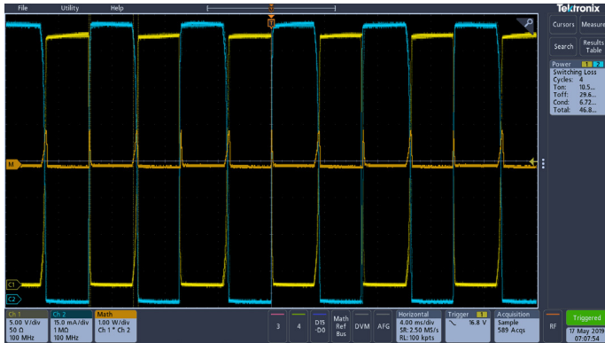
Figure 12. Switching Loss Measurements on an IGBT.
