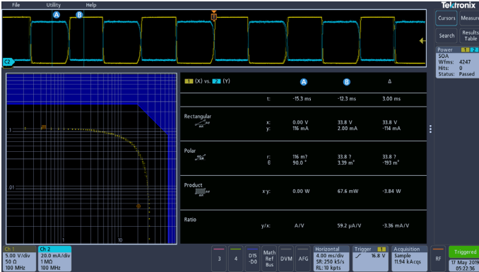
Figure 13. SOA Mask Testing.
